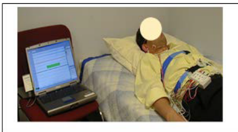
Figure 3. EEG
